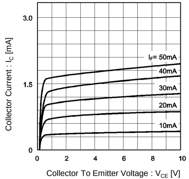
Fig.10 Output Characteristics
